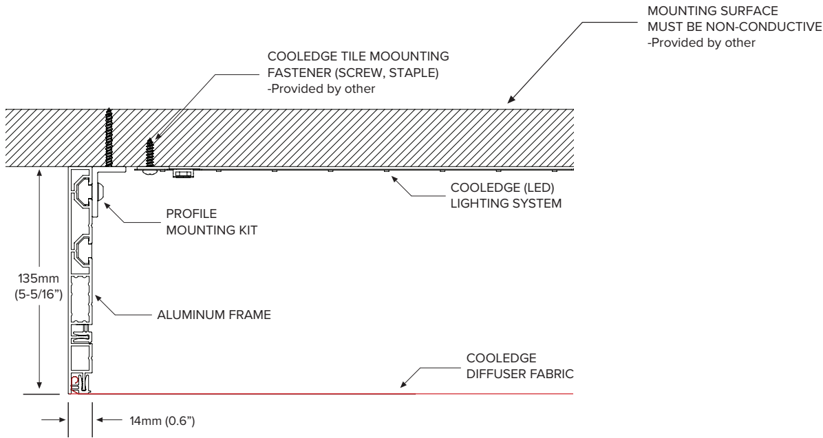
X-Section
